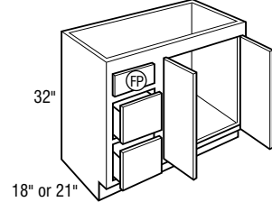
Vanity Sink Drawer Bases, 32" High
